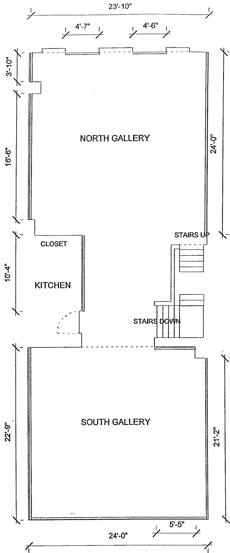
SECOND FLOOR THE PRINT CENTER SCALE 1"=1/8"
